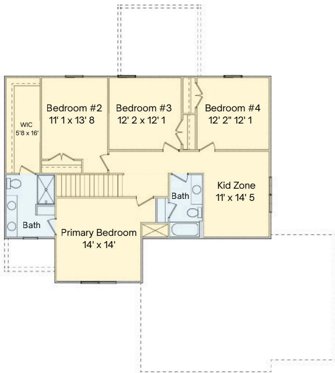
2nd Level Floorplan (Basment Foundation)
