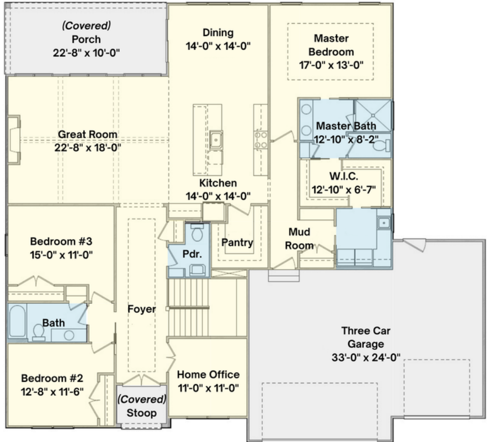
Main Level Floorplan (Basement Foundation)
