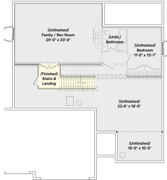
Lower Level Floorplan (Unfinished Basement)
