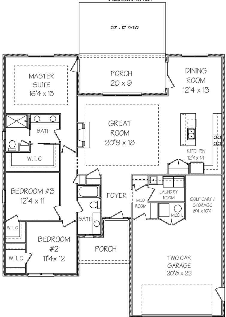
MAIN LEVEL FLOOR PLAN / SLAB OPTION
