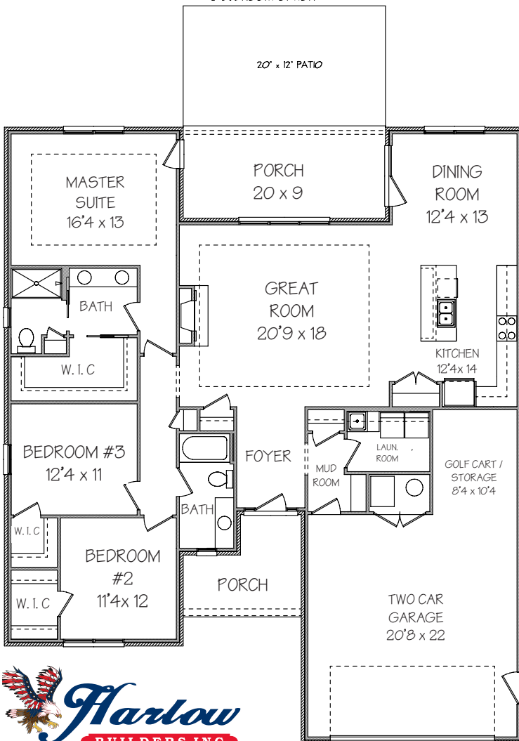
MAIN LEVEL FLOOR PLAN / PARTIAL BASEMENT OPT. 3 BEDROOM OPTION
