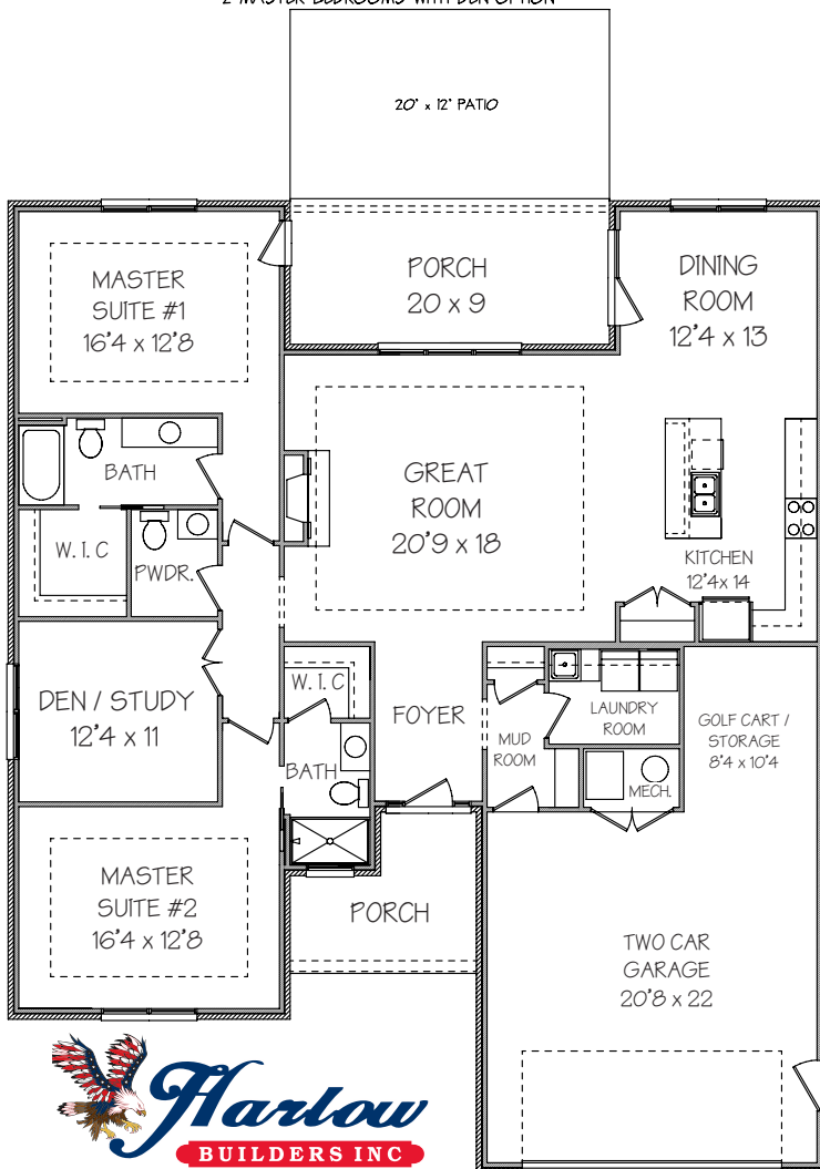
MAIN LEVEL FLOOR PLAN / SLAB OPTION
