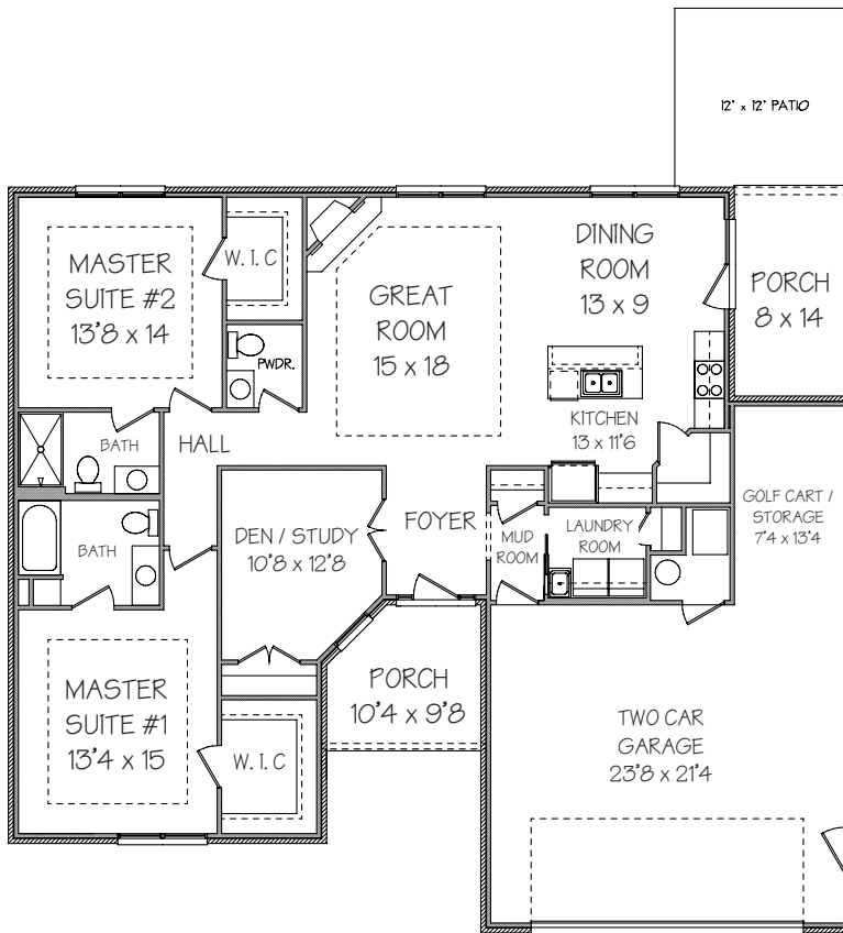
MAIN LEVEL FLOOR PLAN / SLAB OPTION 2 MASTER BEDROOMS WITH DEN OPTION
