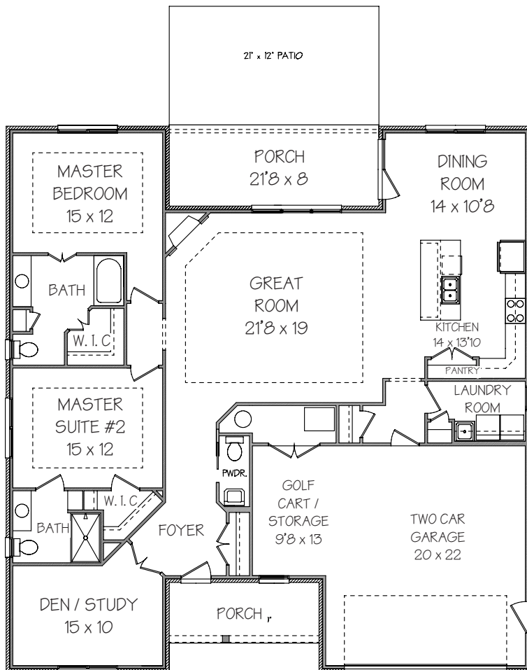
MAIN LEVEL FLOOR PLAN / SLAB OPTION
