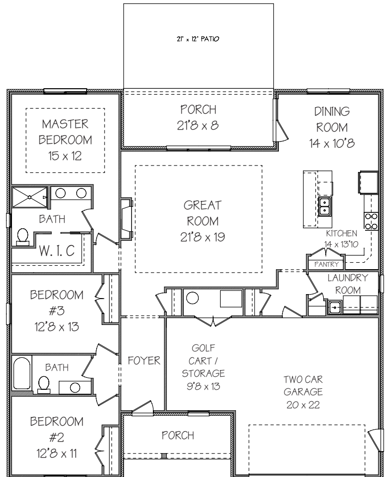
MAIN LEVEL FLOOR PLAN / SLAB OPTION
