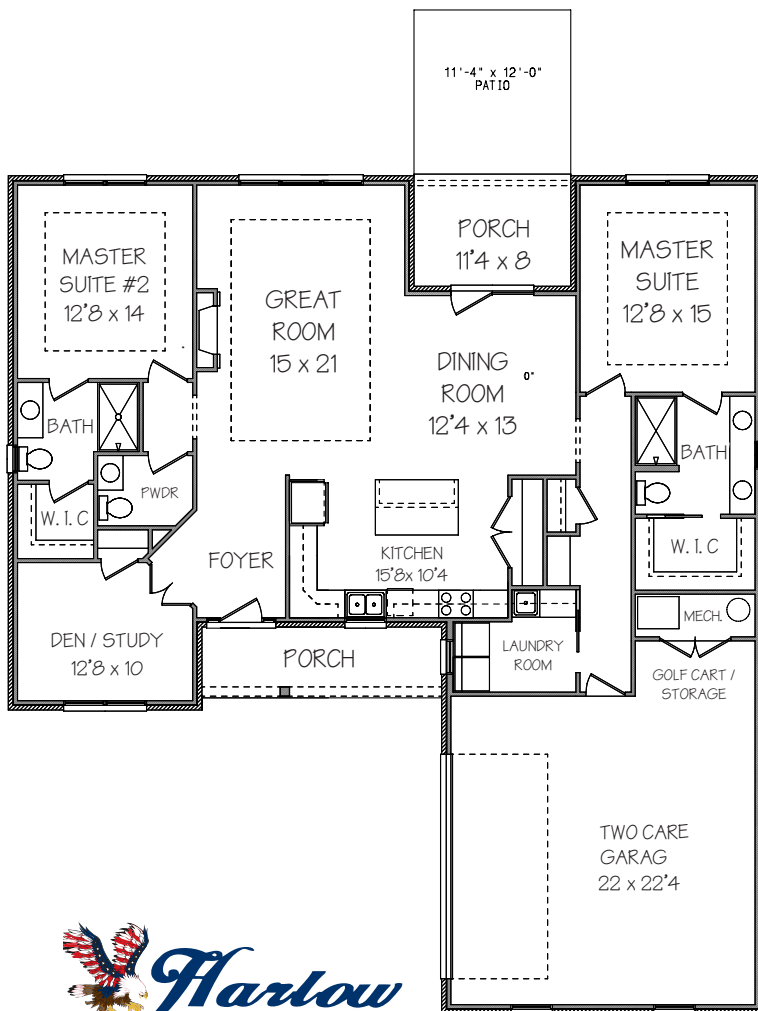
MAIN LEVEL FLOOR PLAN / SLAB OPTION
